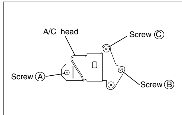
Fig. 2-4-5 A/C head
