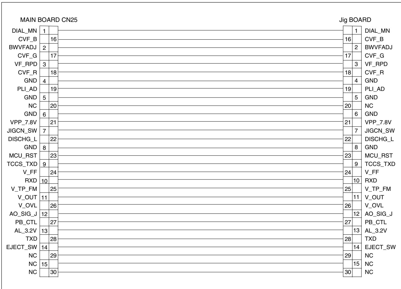
Fig. 2-6-2 Jig connector cable schematic diagram
